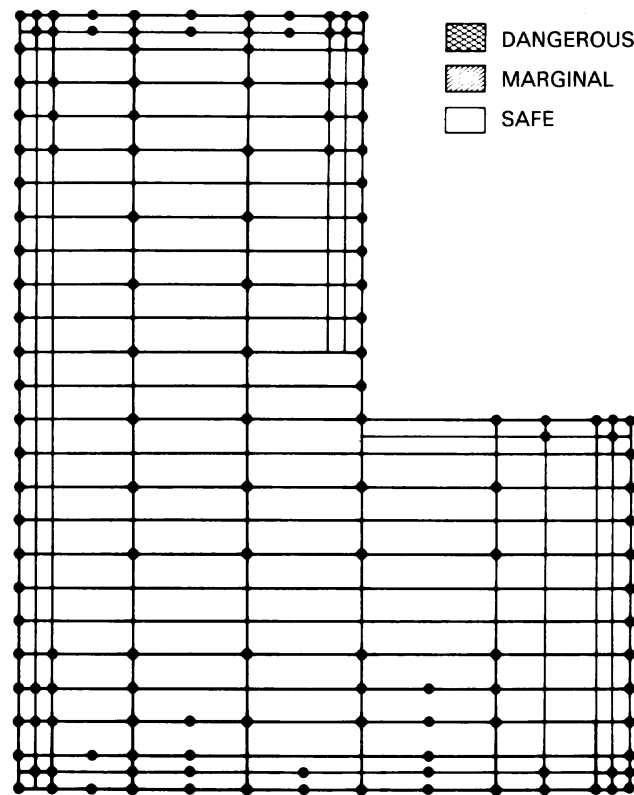
Figure 14-13—Typical ground mat design, final refinement with no hazardous touch potentials
