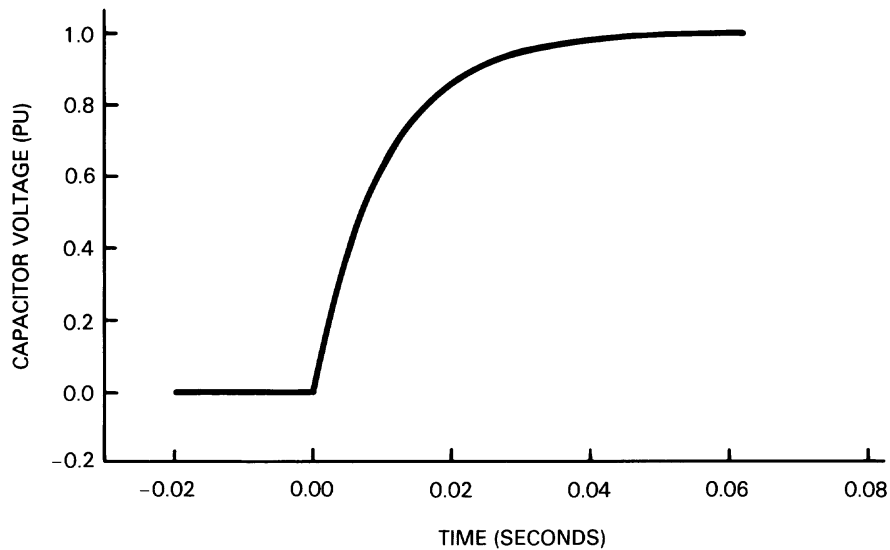
Figure 3-13—Voltage response
