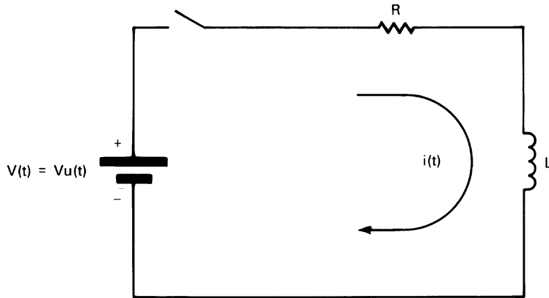
Figure 3-9— RL network
