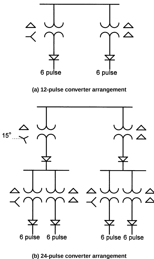
Figure 10-9—Multipulse converter arrangements
